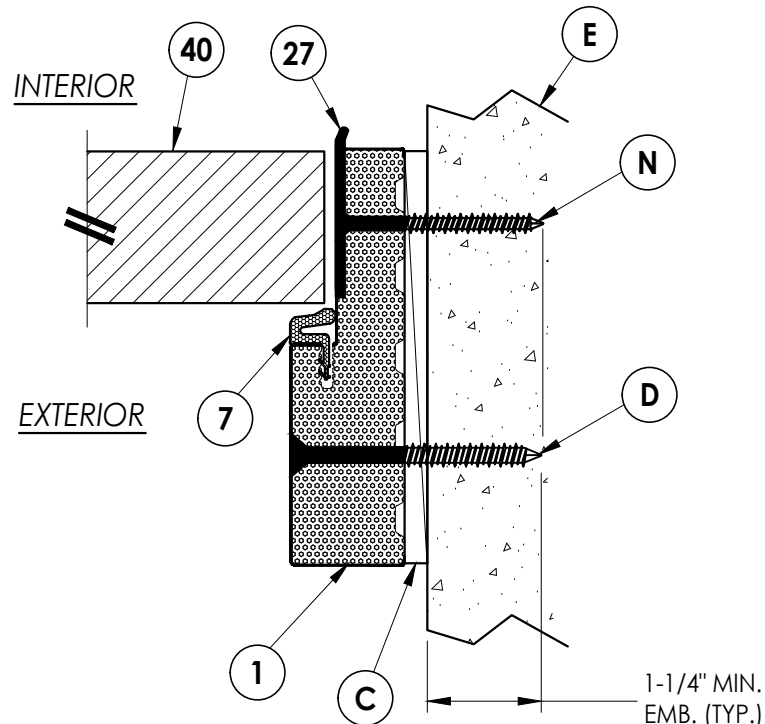
3 3 HORIZONTAL CROSS SECTION Shown Direct to masonry Inswing
