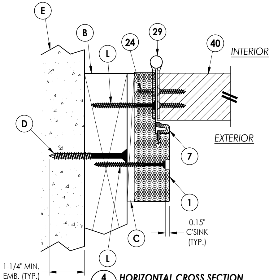
4 3 HORIZONTAL CROSS SECTION Shown with 2X Buck Inswing
