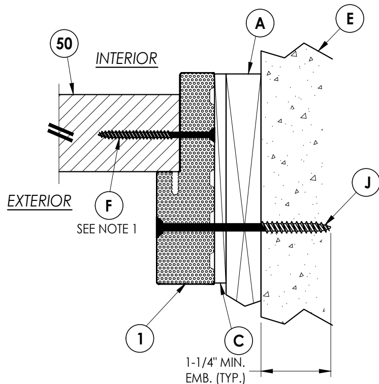
6 3 HORIZONTAL CROSS SECTION Shown with 1X Buck Inswing
