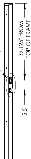
6'8 STRIKE JAMB/MULLION
