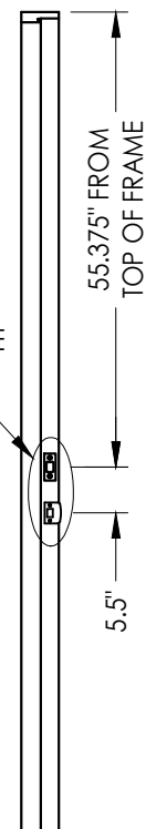
8'0 STRIKE JAMB/MULLION
