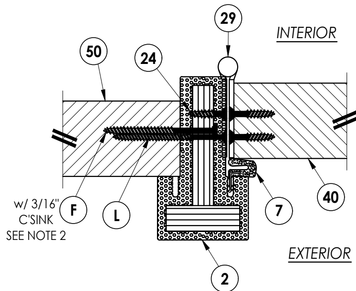
2 3 HORIZONTAL CROSS SECTION Type B (1") Integral Mullion Inswing
