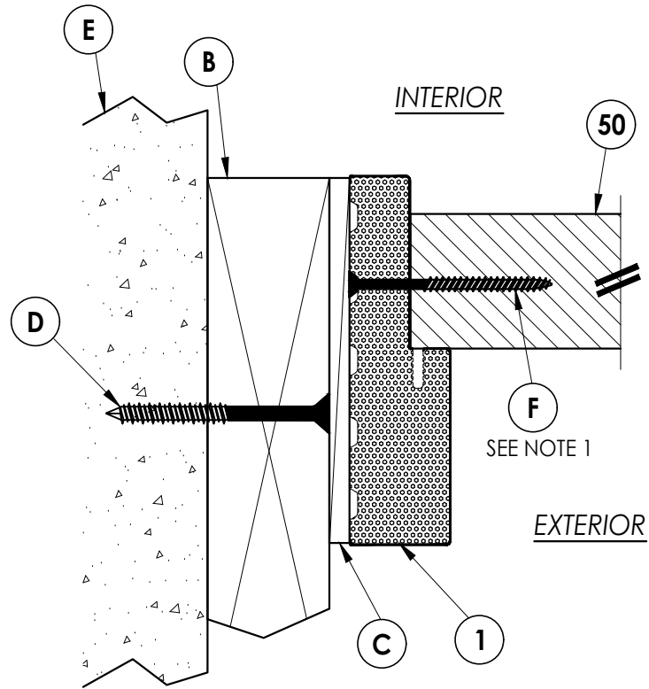
1 3 HORIZONTAL CROSS SECTION Shown with 2X Buck Inswing
