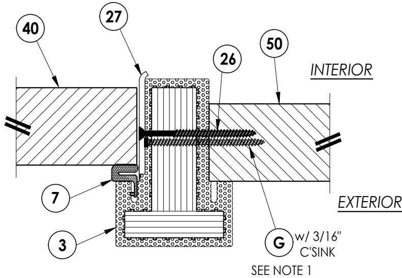
3 3 HORIZONTAL CROSS SECTION Shown Direct to masonry Inswing
